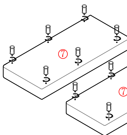
BOXSPRING LEGS INSTALLATION
