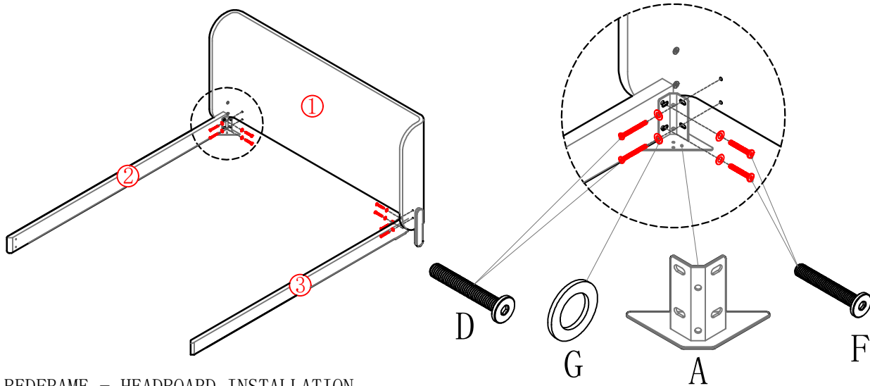
BEDFRAME - HEADBOARD INSTALLATION
