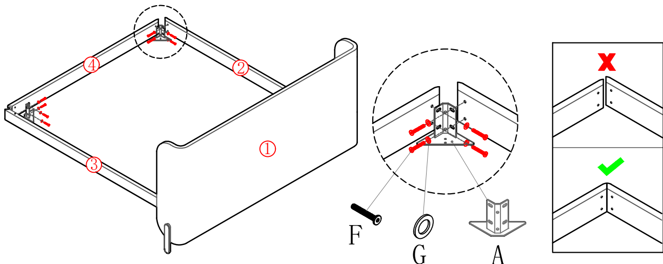
DECORATIVE LEGS INSTALLATION
