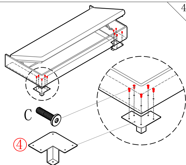
CORNER METAL LEGS INSTALLATION
