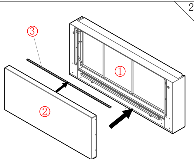
UPPER - LOWER BOX INSTALLATION
